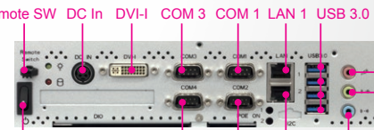
Power Button COM 4 COM 2 LAN 2 Line In
