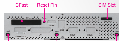
Antenna Hole Antenna Hole Antenna Hole
